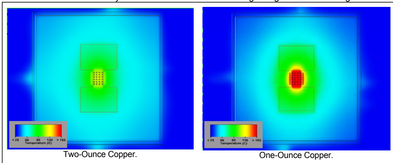
Figure 6. Thermal gradients of a PowerSO on a 5 in. x 5 in. two-sided board vs. copper foil thickness.
