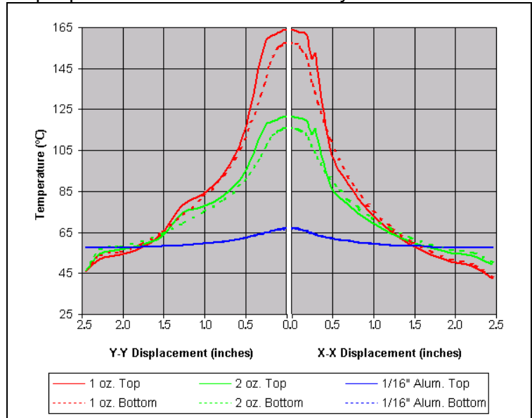
Figure 8. Thermal Gradients of Some 5 in. x 5 in. Materials
