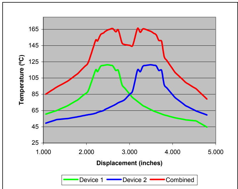
Figure 10. Heat Rise Of Two PowerSOs Placed One Inch Apart
