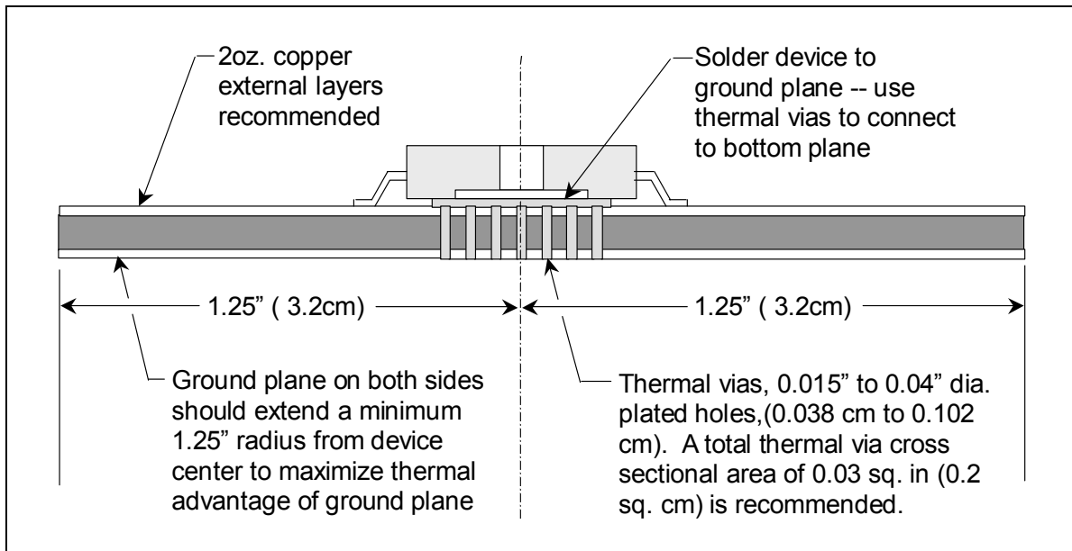
Figure 2. Typical PowerSO PC Board Mounting.
